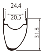
JETFLY DISC ASYMMETRIC RIM
